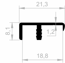
JM 1070 BORDER COVERING WEIGHT : 0,150 kg/m
