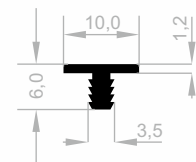
JM 4653 BORDER COVERING WEIGHT : 0,199 kg/m
