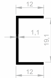
JM 4624 BORDER COVERING WEIGHT : 0,129 kg/m
