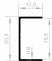
JM 8531 BORDER COVERING WEIGHT : 0,088 kg/m
