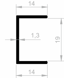
JM 4514 BORDER COVERING WEIGHT : 0,169 kg/m
