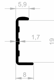
JM 4581 BORDER COVERING WEIGHT : 0,112 kg/m
