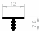
JM 1067 BORDER COVERING WEIGHT : 0,145 kg/m
