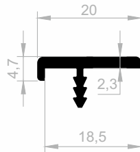
JM 4324 BORDER COVERING WEIGHT : 0,175 kg/m
