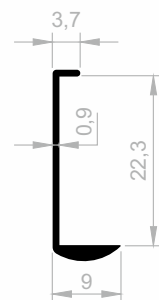
JM 6231 BORDER COVERING WEIGHT : 0,101 kg/m
