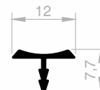
JM 4656 BORDER COVERING WEIGHT : 0,170 kg/m
