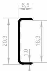
JM 3475 BORDER COVERING WEIGHT : 0,067 kg/m
