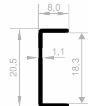
JM 2979 BORDER COVERING WEIGHT : 0,100 kg/m
