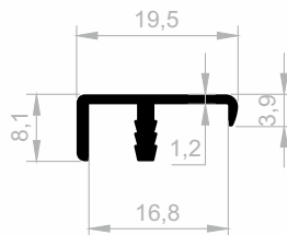
JM 1067 BORDER COVERING WEIGHT : 0,145 kg/m
