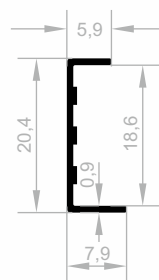
JM 1926 BORDER COVERING WEIGHT : 0,087 kg/m
