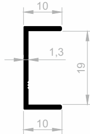
JM 4598 BORDER COVERING WEIGHT : 0,140 kg/m
