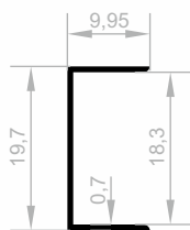
JM 3475 BORDER COVERING WEIGHT : 0,067 kg/m
