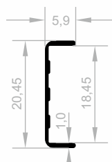
JM 8547 BORDER COVERING WEIGHT : 0,069 kg/m
