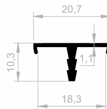
JM 6231 BORDER COVERING WEIGHT : 0,101 kg/m
