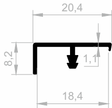
JM 1091 BORDER COVERING WEIGHT : 0,105 kg/m
