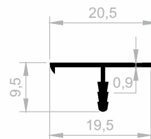
JM 1123 BORDER COVERING WEIGHT : 0,075 kg/m
