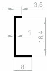
JM 1113 BORDER COVERING WEIGHT : 0,080 kg/m
