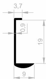
JM 6233 BORDER COVERING WEIGHT : 0,093 kg/m
