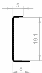
JM 6233 BORDER COVERING WEIGHT : 0,093 kg/m
