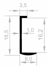
JM 8531 BORDER COVERING WEIGHT : 0,088 kg/m
