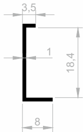
JM 1146 BORDER COVERING WEIGHT : 0,085 kg/m
