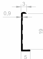
JM 6232 BORDER COVERING WEIGHT : 0,062 kg/m
