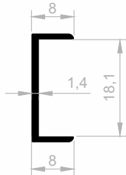
JM 1507 BORDER COVERING WEIGHT : 0,135 kg/m
