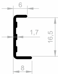
JM 1781 BORDER COVERING WEIGHT : 0,090 kg/m
