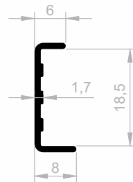
JM 1089 BORDER COVERING WEIGHT : 0,115 kg/m
