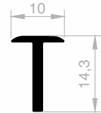
JM 5756 BORDER COVERING WEIGHT : 0,101 kg/m
