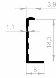
JM 5698 BORDER COVERING WEIGHT : 0,085 kg/m
