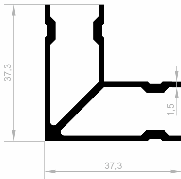
JM 1784 SHELF PROFILE WEIGHT : 0,661 kg/m
