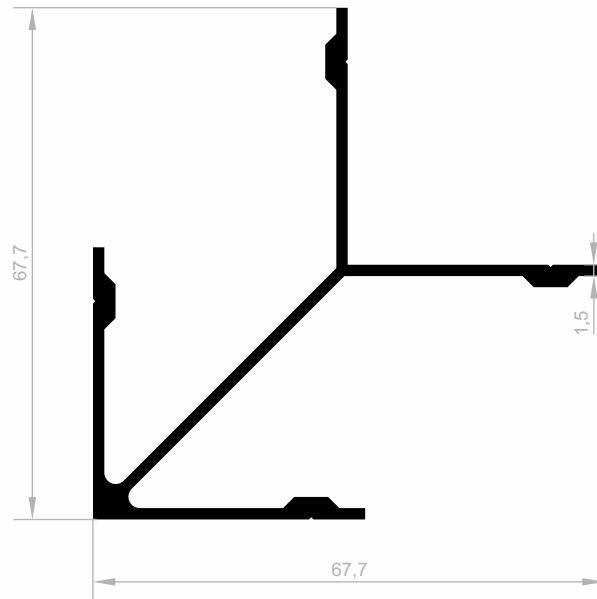
JM 1783 SHELF PROFILE WEIGHT : 0,854 kg/m
