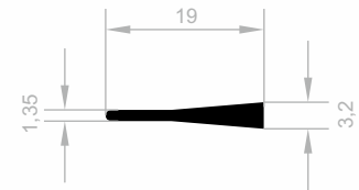
J 1670 SPECIAL PROFILES WEIGHT : 0,097 kg/m
