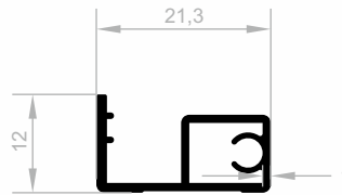
J 1133 SPECIAL PROFILES WEIGHT : 0,189 kg/m
