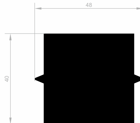
J 8774 SPECIAL PROFILES WEIGHT : 4,386 kg/m
