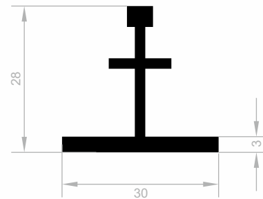
J 1680 SPECIAL PROFILES WEIGHT : 0,466 kg/m
