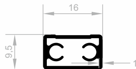
J 1132 SPECIAL PROFILES WEIGHT : 0,173 kg/m
