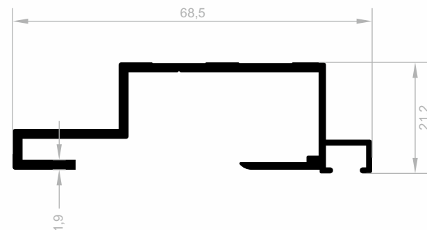
J 1061 SPECIAL PROFILES WEIGHT : 0,632 kg/m
