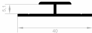
J 3175 SPECIAL PROFILES WEIGHT : 0,251 kg/m
