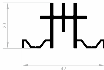
J 3335 SPECIAL PROFILES WEIGHT : 0,501 kg/m
