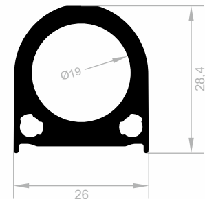
J 10288 SPECIAL PROFILES WEIGHT : 0,862 kg/m
