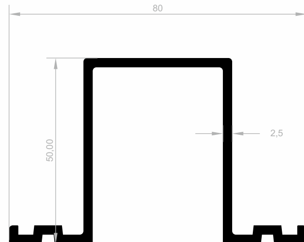
J 1519 SPECIAL PROFILES WEIGHT : 1,279 kg/m
