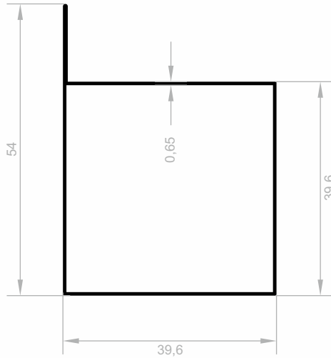
J 8573 SPECIAL PROFILES WEIGHT : 0,309 kg/m
