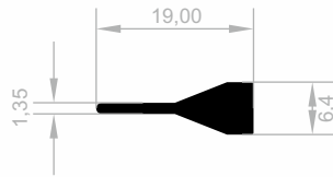
J 1671 SPECIAL PROFILES WEIGHT : 0,154 kg/m
