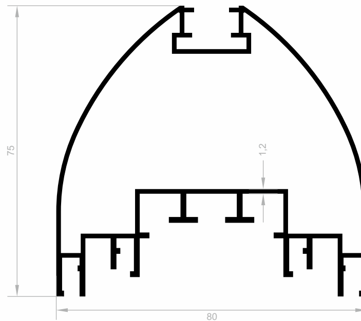
J 1239 SPECIAL PROFILES WEIGHT : 1,488 kg/m
