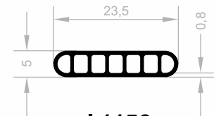
J 1156 SPECIAL PROFILES WEIGHT : 0,150 kg/m
