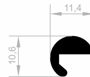
J 1246 SPECIAL PROFILES WEIGHT : 0,148 kg/m
