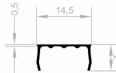
J 2196 SPECIAL PROFILES WEIGHT : 0,049 kg/m
