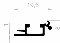
J 1161 DISPLAY PROFILE WEIGHT : 0,330 kg/m
