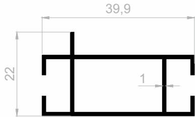
J 1964 DISPLAY PROFILE WEIGHT : 0,354 kg/m
