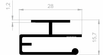
J 1204 DISPLAY PROFILE WEIGHT : 0,300 kg/m
