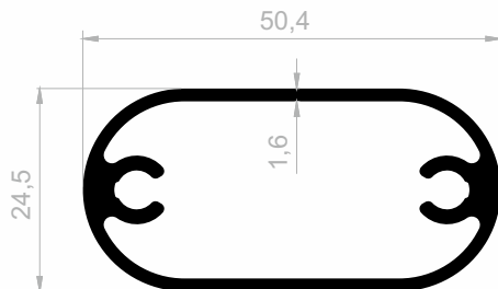
J 2879 DISPLAY PROFILE WEIGHT : 0,726 kg/m
