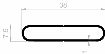
J 1202 DISPLAY PROFILE WEIGHT : 0,216 kg/m
