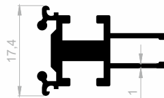
J 1161 DISPLAY PROFILE WEIGHT : 0,330 kg/m
