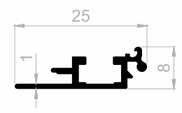
J 1204 DISPLAY PROFILE WEIGHT : 0,300 kg/m
