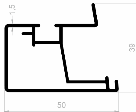
J 1512 DISPLAY PROFILE WEIGHT : 0,751 kg/m
