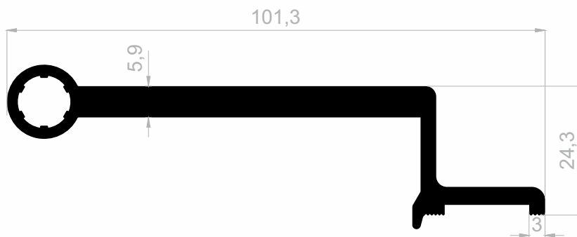
J 1620 HINGE PROFILES WEIGHT : 1,672 kg/m
