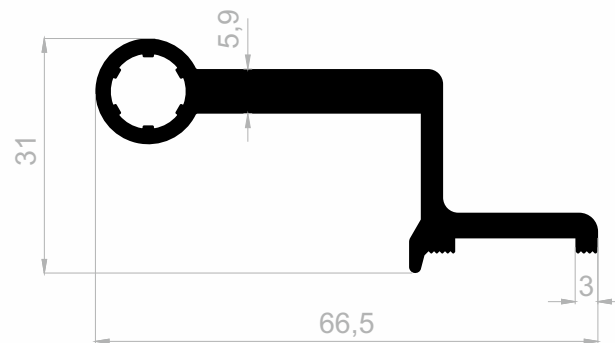
J 1624 HINGE PROFILES WEIGHT : 1,114 kg/m
