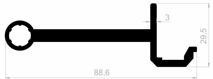
J 1622 HINGE PROFILES WEIGHT : 1,499 kg/m
