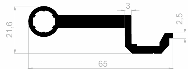
J 1623 HINGE PROFILES WEIGHT : 1,019 kg/m
