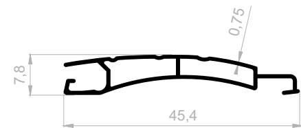
J 3191 ROLLER SHUTTTTERS WEIGHT : 0,219 kg/m
