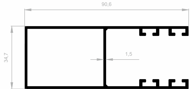
J 3403 ROLLER SHUTTTTERS WEIGHT : 1,225 kg/m
